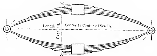
Fig. 5231. DIAGRAM OF ELLIPTIC-SPRING, Showing dimensions required by manufacturers.
